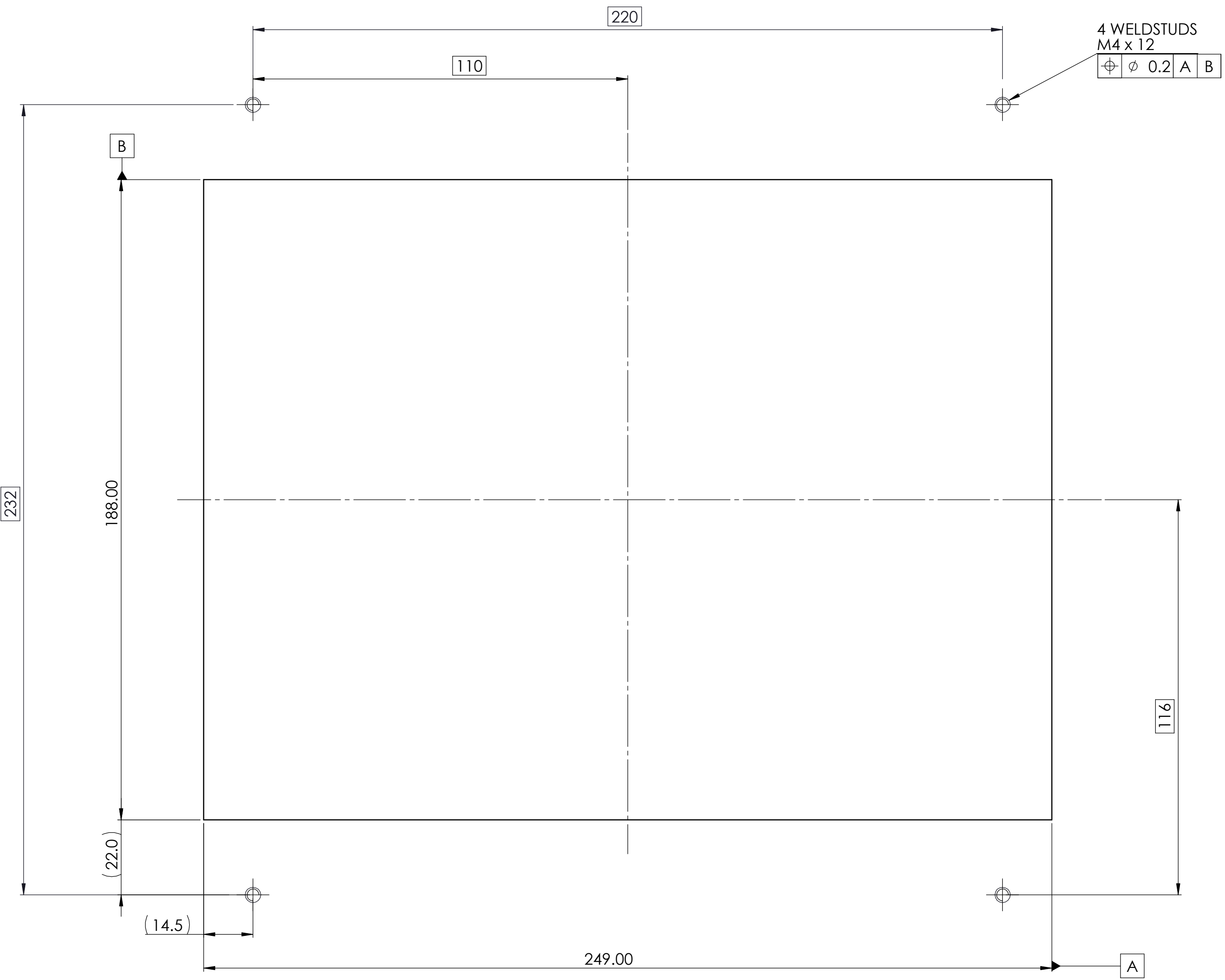
AS VIEWED FROM BACK OF FACEPLATE
