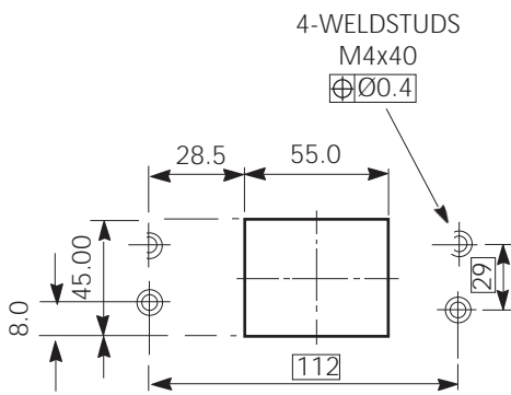
ULS32 HORIZONTAL CUTOUTS
