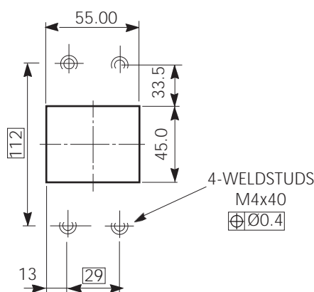
ULS32 VERTICAL CUTOUTS
