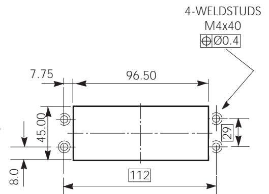
ULS34 HORIZONTAL CUTOUTS
